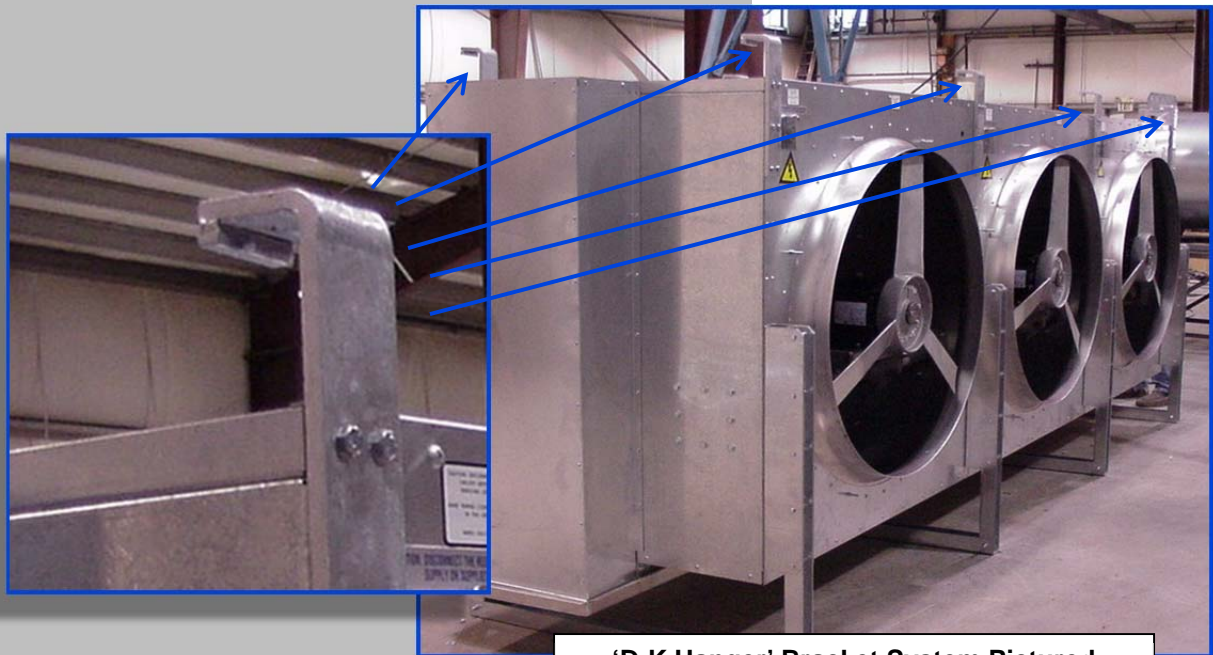
'D-K Hanger' Bracket System Pictured On Doubl-Kold ICH Evaporator
